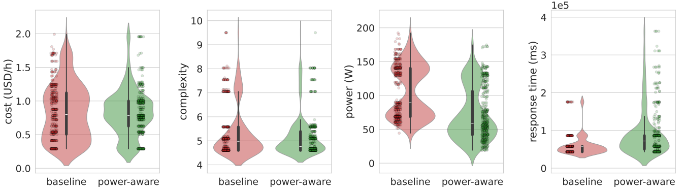
Fig. 3. Distributions of the objective values in the baseline and the power-aware experiments. Plotted solutions are all the Pareto fronts obtained in the 31 runs.
